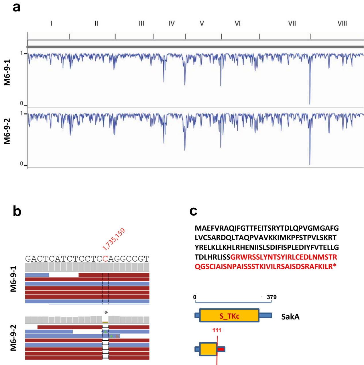
Suppl. Figure S3: Identification of the mutation in the mutant M6-9 by whole genome sequencing. (a) Coverage analysis shows that the genomes of M6-9-1 (only background mutations) and M6-9-2 (putative phenotype-causing mutation and background mutations) are identical. No big deletions or insertions were observed. (b) A 1 nt deletion was detected in the sakA gene. (c) The translated protein of the mutated sakA gene lacks the kinase domain.
